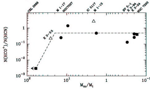
Fig. 2. Abundance of HCO + relative to HCN as a function of M_{mol}/M_{HII} \sim 25 . All points but K3-35 are from Josselin & Bachiller (2003)
