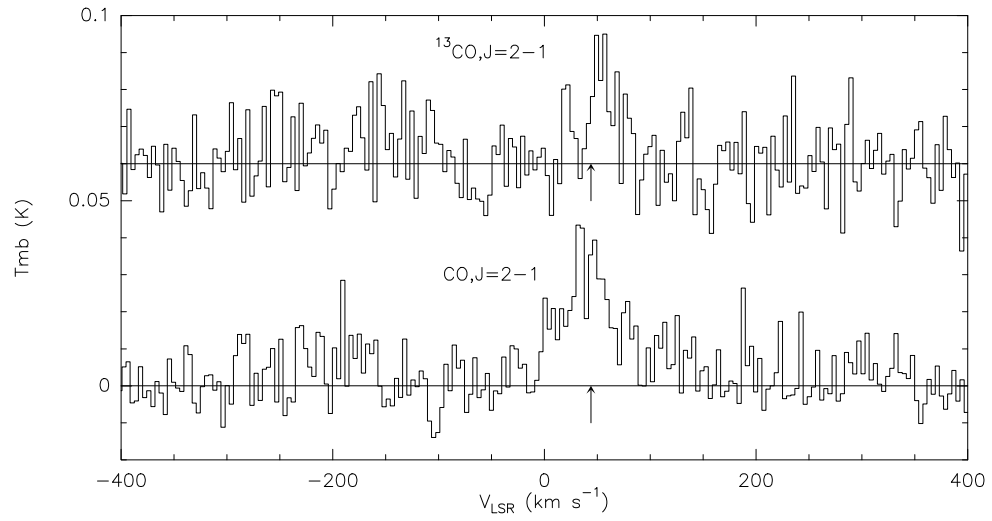
Fig. 1. The observed ^{12}\text{CO} and ^{13}\text{CO} 2–1 line profiles. The spectra have been box smoothed to a resolution of about 3 MHz. The ^{13}\text{CO} 2–1 line has been shifted upward by 0.06 K for clarity. The arrows mark V_{\text{sys}} = 44 \text{ km s}^{-1} that is derived from the ^{12}\text{CO} line.
