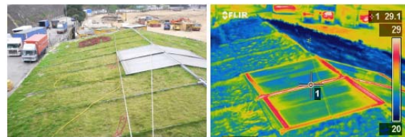
Figure 6. Infrared thermograph of the green roof.
