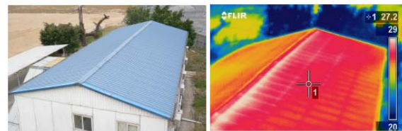
Figure 7. Infrared thermograph of a conventional roof.
