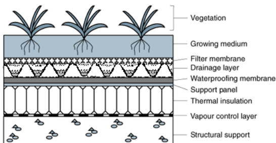
Figure 1. Typical structure of extensive green roof.
