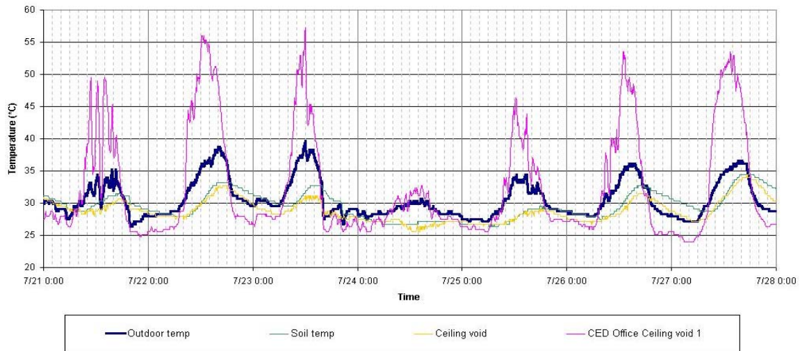
Figure 5. Results of the temperature measurements.
